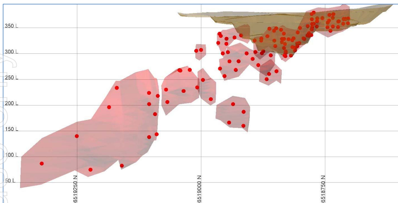
Figure 16 - Long section of 132N looking east with drill pierce points within modelled nickel mineralisation. Future work should include structurally orientated diamond core, and infill drilling to increase confidence in the Mineral Resource
