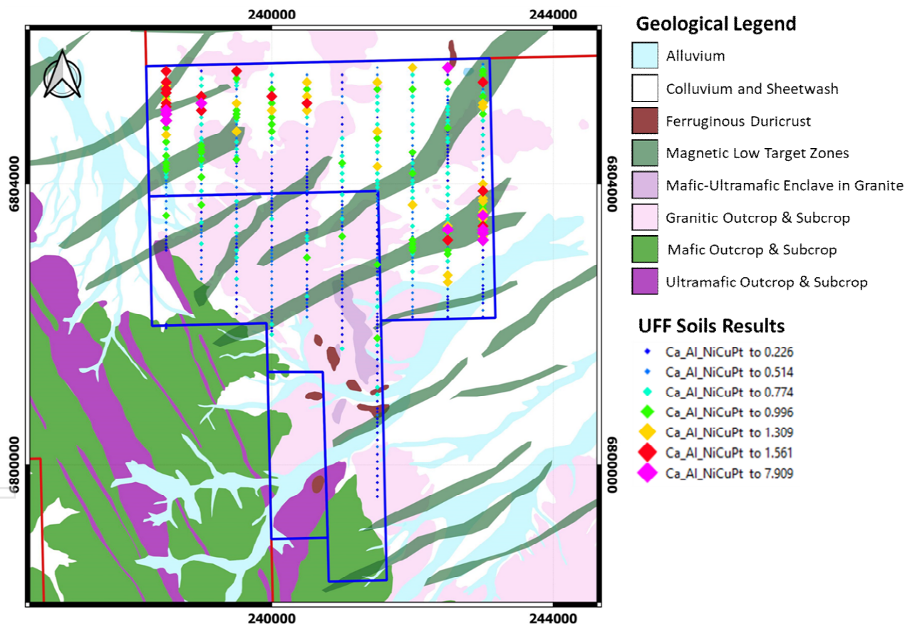
Figure 5 Data has been Ca-Normalised. Data shown as additive Index (Ni, Cu & Pt)
