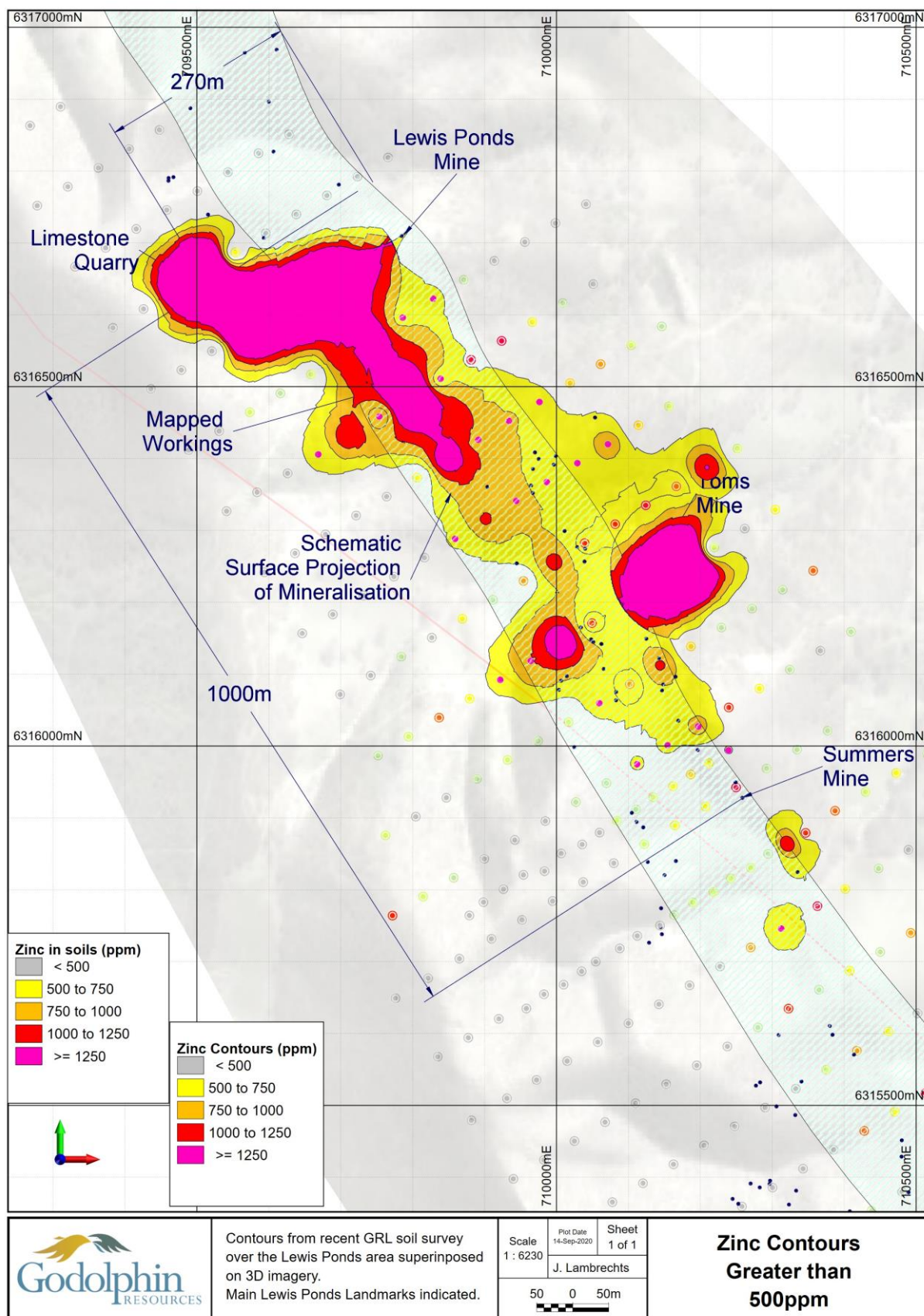
Appendix 4: Map of the zinc contours at Lewis Ponds generated from the recent soil sample results
