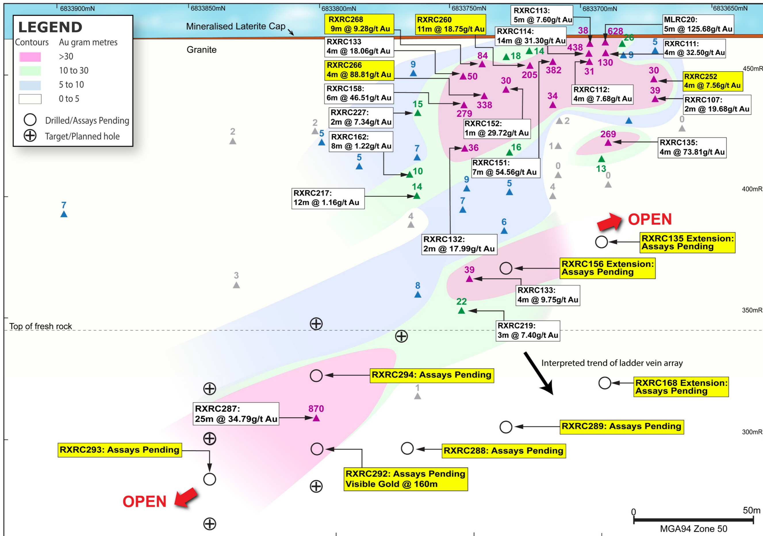
Figure 2 - Grace Prospect Long Section
