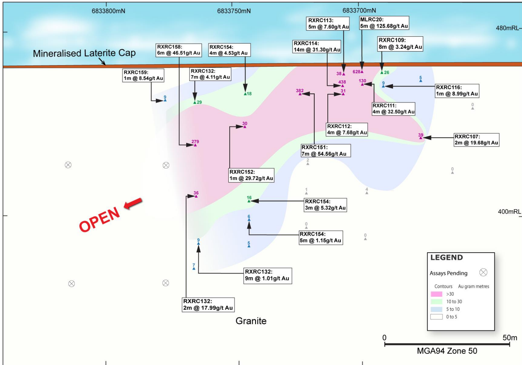
Figure 2 – Grace Prospect Long Section
