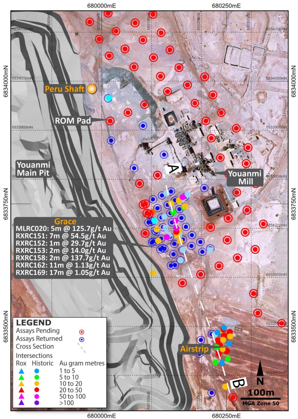
Figure 1 – Grace & Youanmi South Plan
