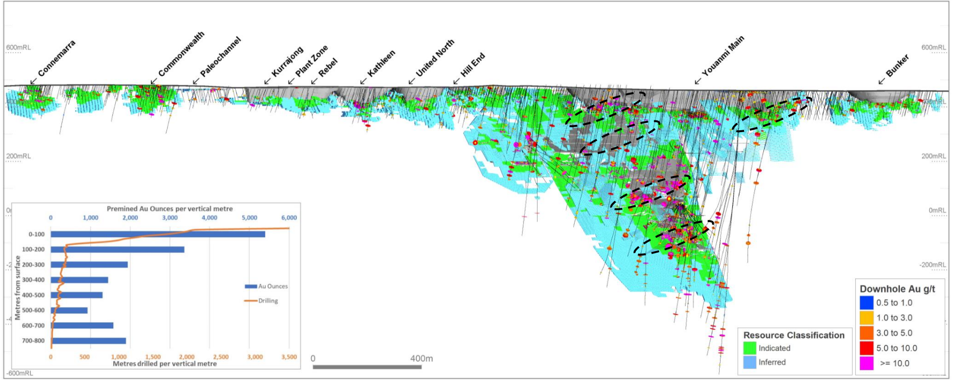
Figure 4 – Long Section through Main Lode at Youanmi (i.e west of Grace section) showing historical workings and interpreted northerly plunging very high-grade shoots within steep south plunging ore zone
