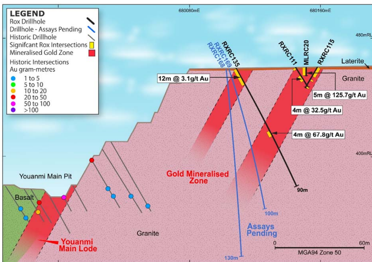
Figure 2 - Cross Section A - Main Pit and Grace Prospect showing depth extension and new HW mineralisation
