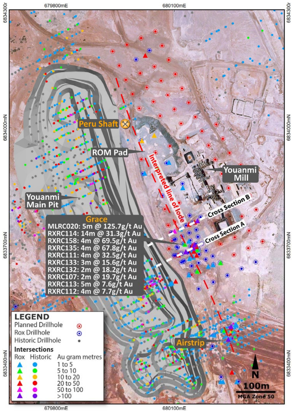
Figure 2 – Grace Prospect drill pierce points (gram metre intersections) and planned drill collars
