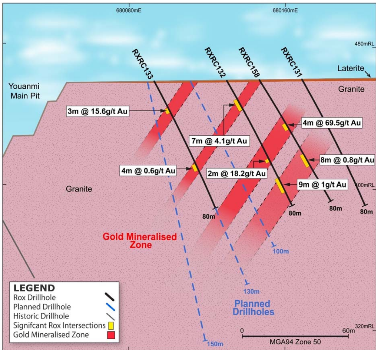
Figure 3 - Cross Section B - Main Pit and Grace Prospect showing depth extension and new HW mineralisation
