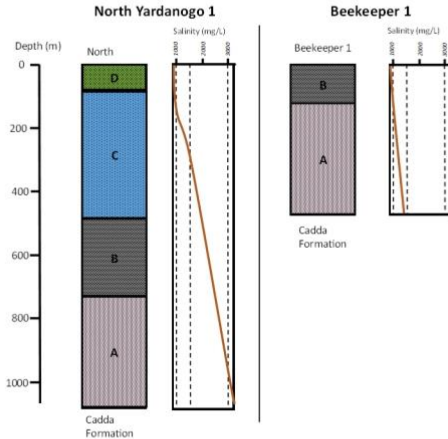
Figure 43: Geological profile: sub-division units (A-D) and interpretive groundwater salinity (Through the Yarragadee Formation within North Yordanogo 1 and Beekeeper 1)
