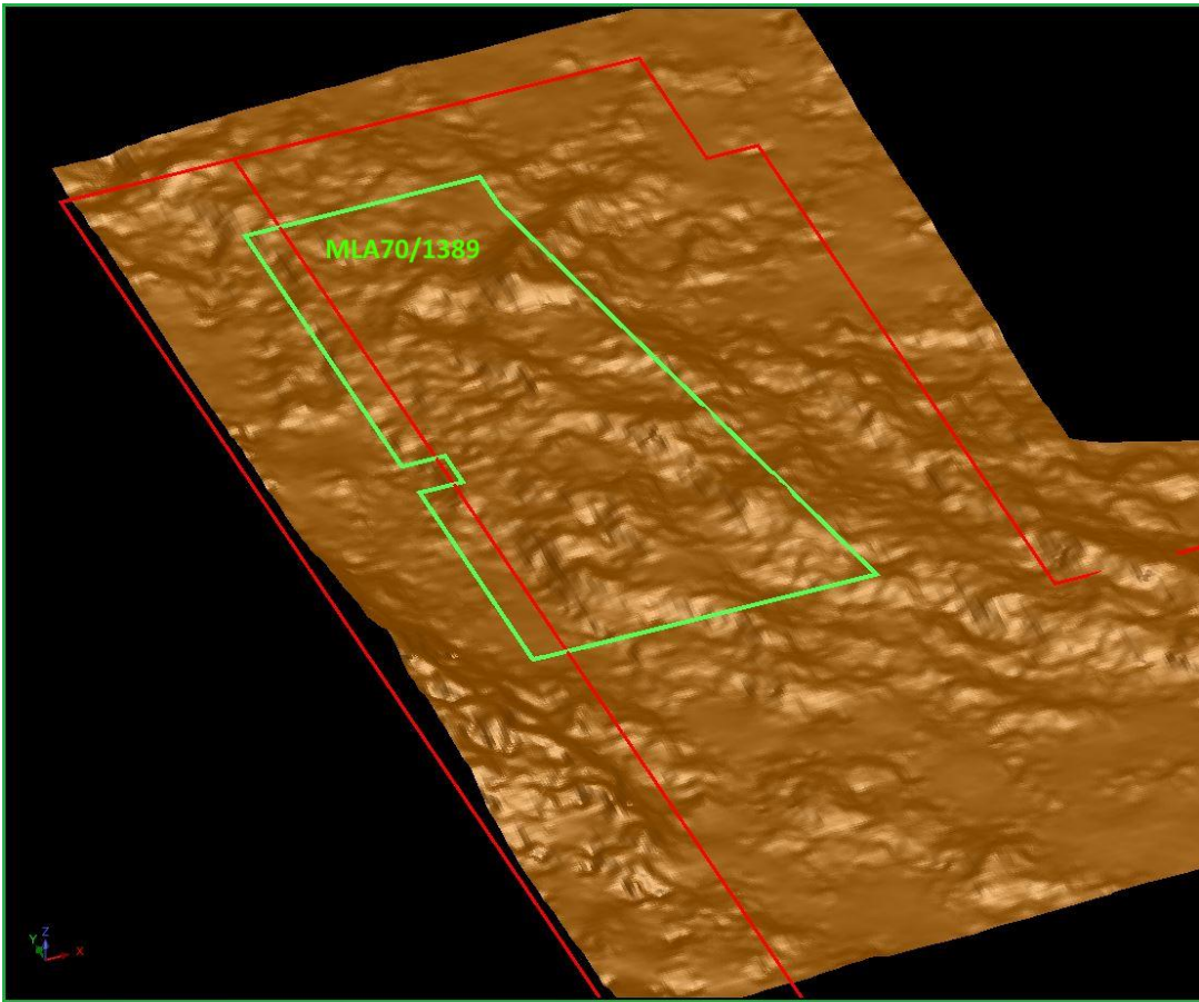
Figure 13: Arrowsmith North Pre-Mining Topography (10:1 vertical exaggeration)
