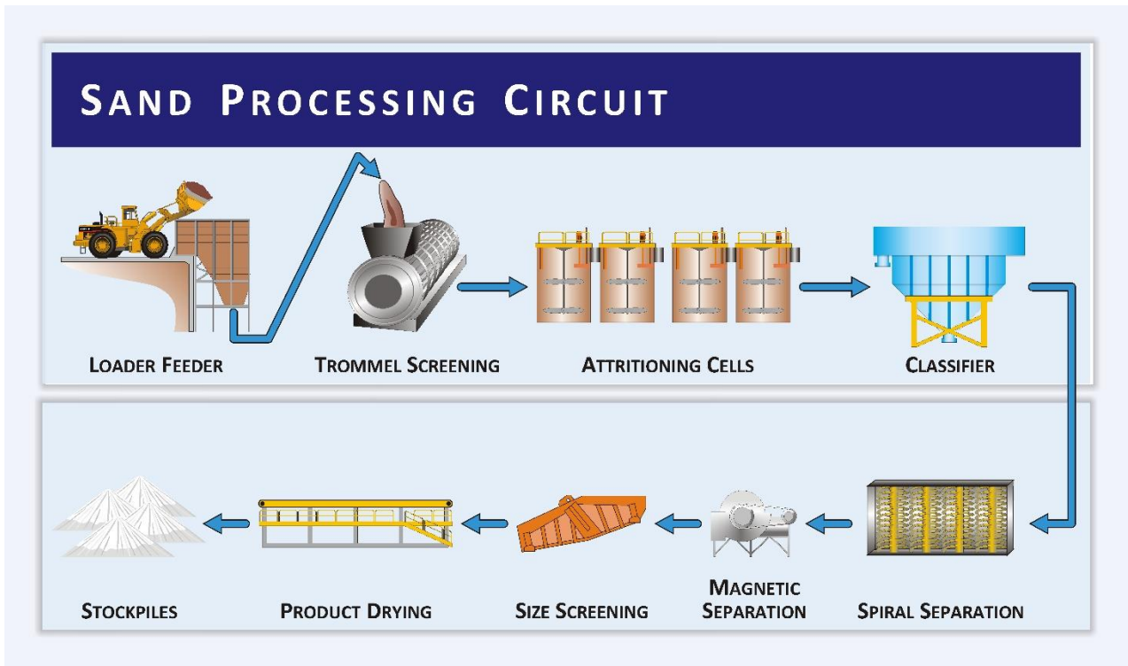
Figure 34: Processing circuit
