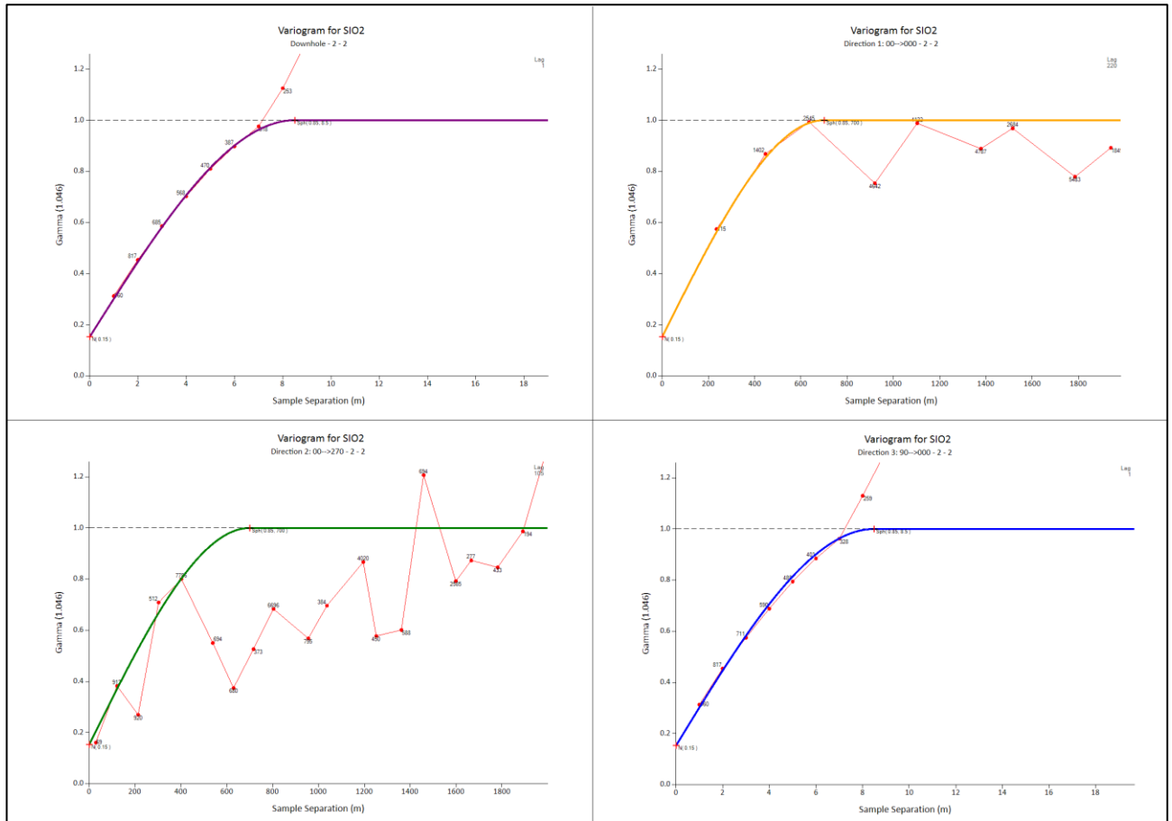
Figure 10: Variogram models
