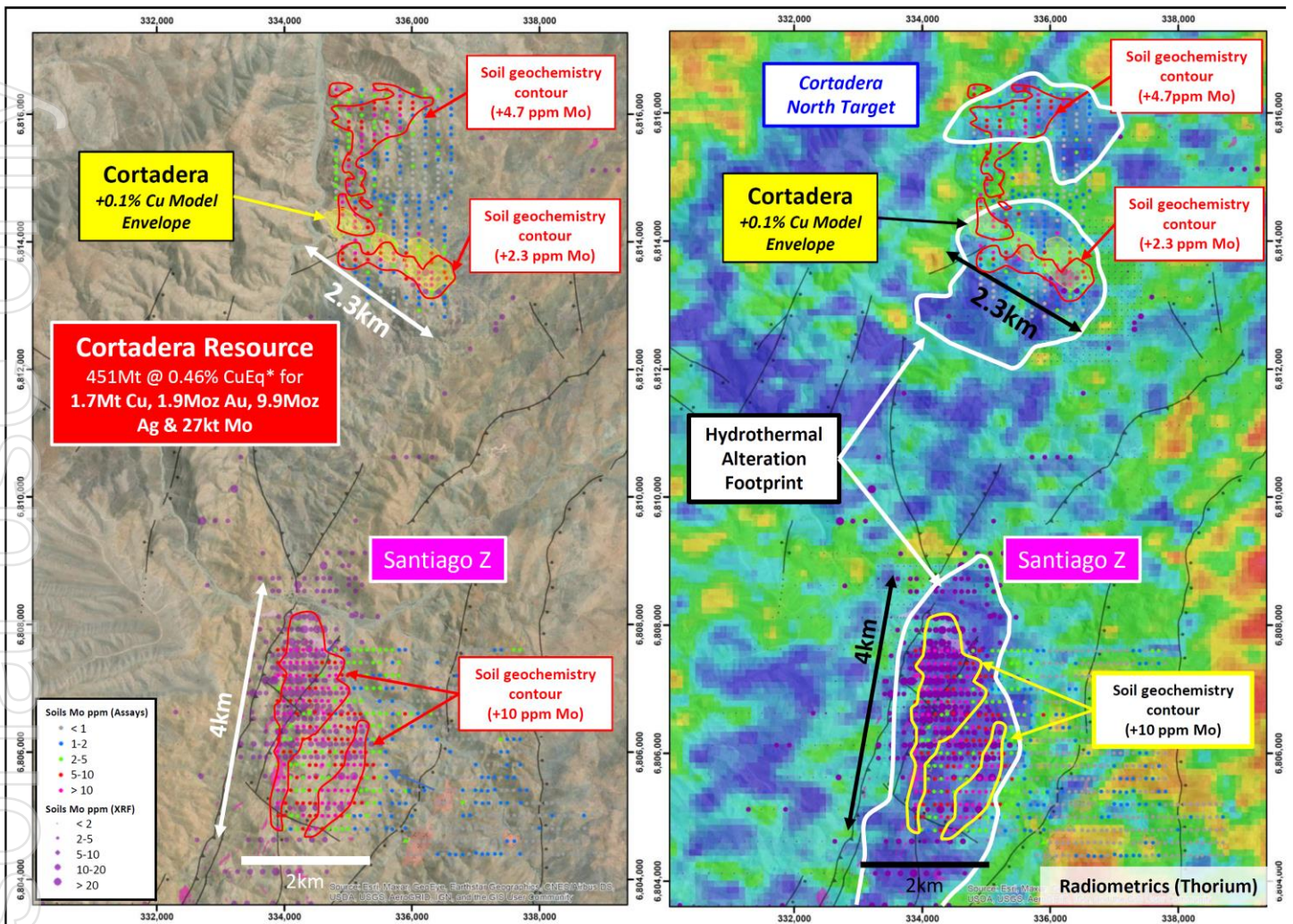
Figure 2. Location of the Santiago Z soil molybdenum footprint, 5km south of the Cortadera Cu-Au discovery
