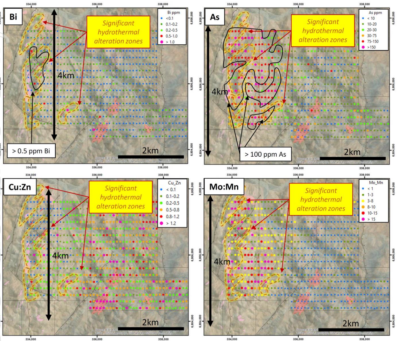
Figure 4. New soil geochemistry results for other pathfinder elements and metal zonation patterns across the Santiago Z copper porphyry alteration footprint
