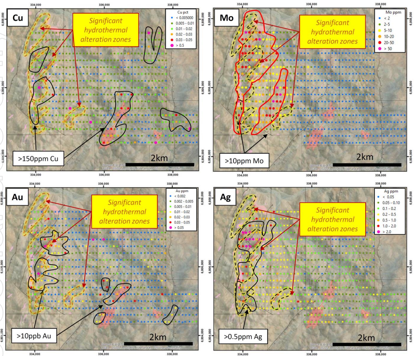
Figure 3. New soil geochemistry results for copper, gold, molybdenum and silver across the Santiago Z copper porphyry alteration footprint
